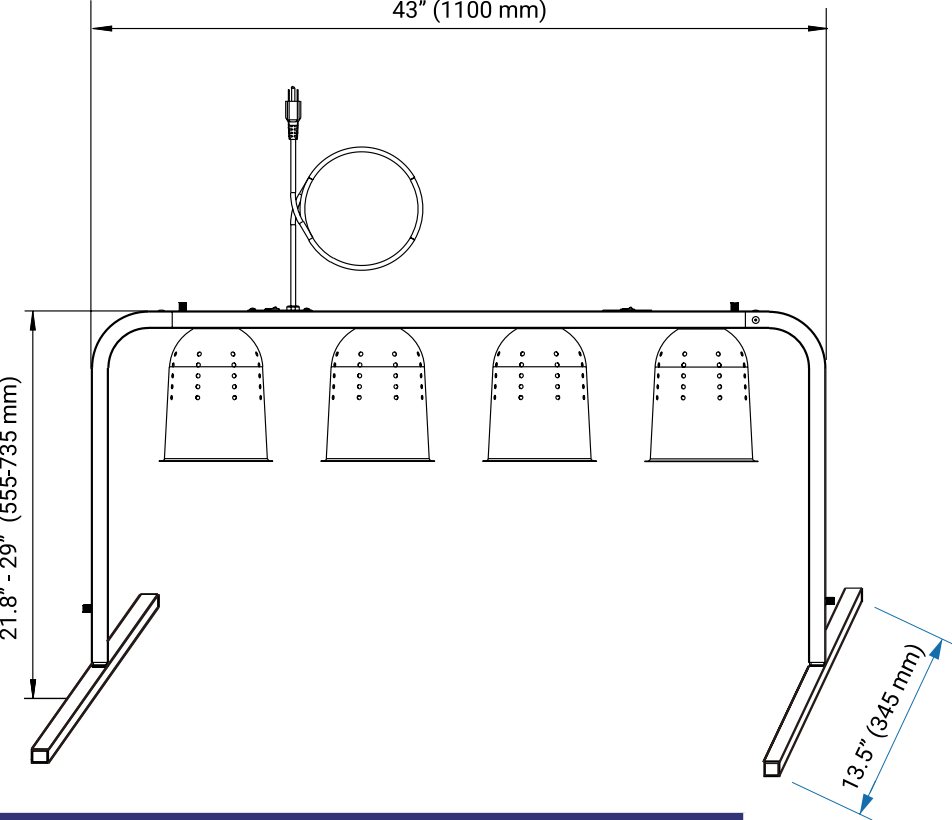
TECHNICAL DRAWING (48396)
