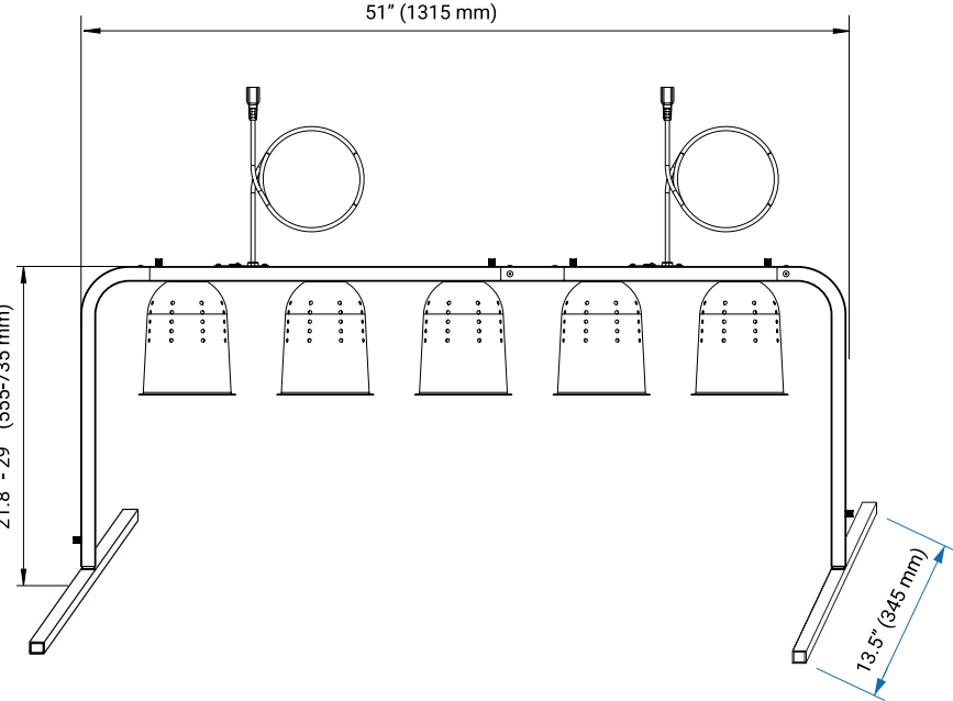
TECHNICAL DRAWING (48396)
